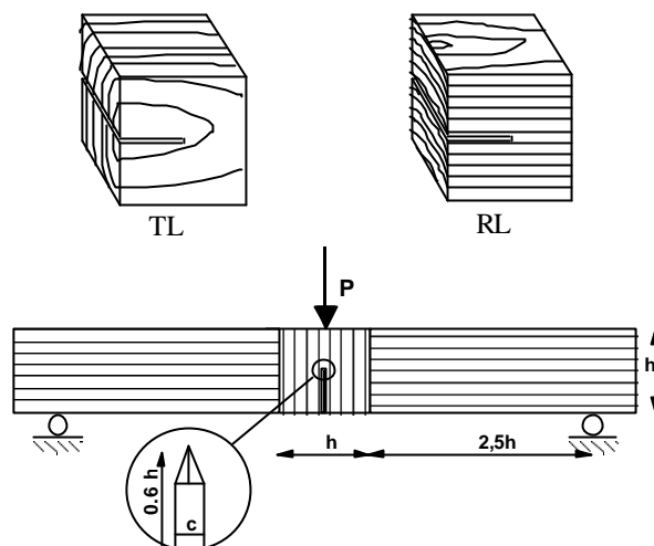
Figure 1 - Essai de flexion trois points Three point bending test
